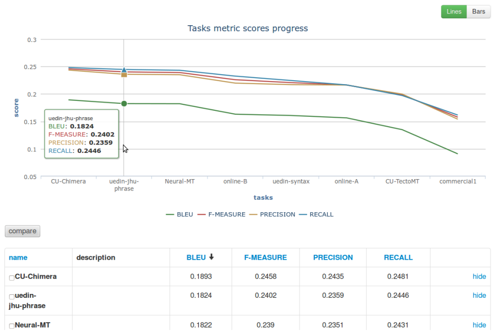
Figure 2. Listing of tasks of the “Newstest 2015 en-cs” experiment at wmt.ufal.cz.
