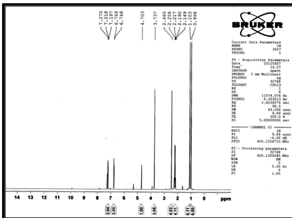
9-(4-Methoxy)-3,3,6,6-tetramethyl-1,2,3,4,5,6,7,8-octahydroanthene-1,8-dione:
