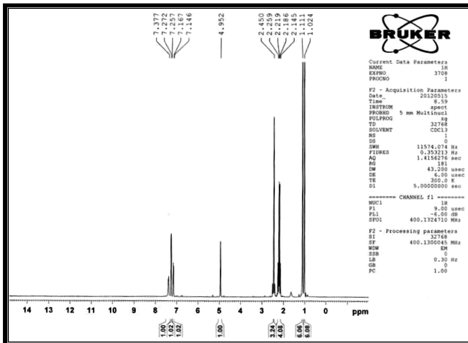
9-(2,4-Dichlorophenyl)-3,3,6,6-tetramethyl-1,2,3,4,5,6,7,8-octahydroxanthene-1,8-dione:
