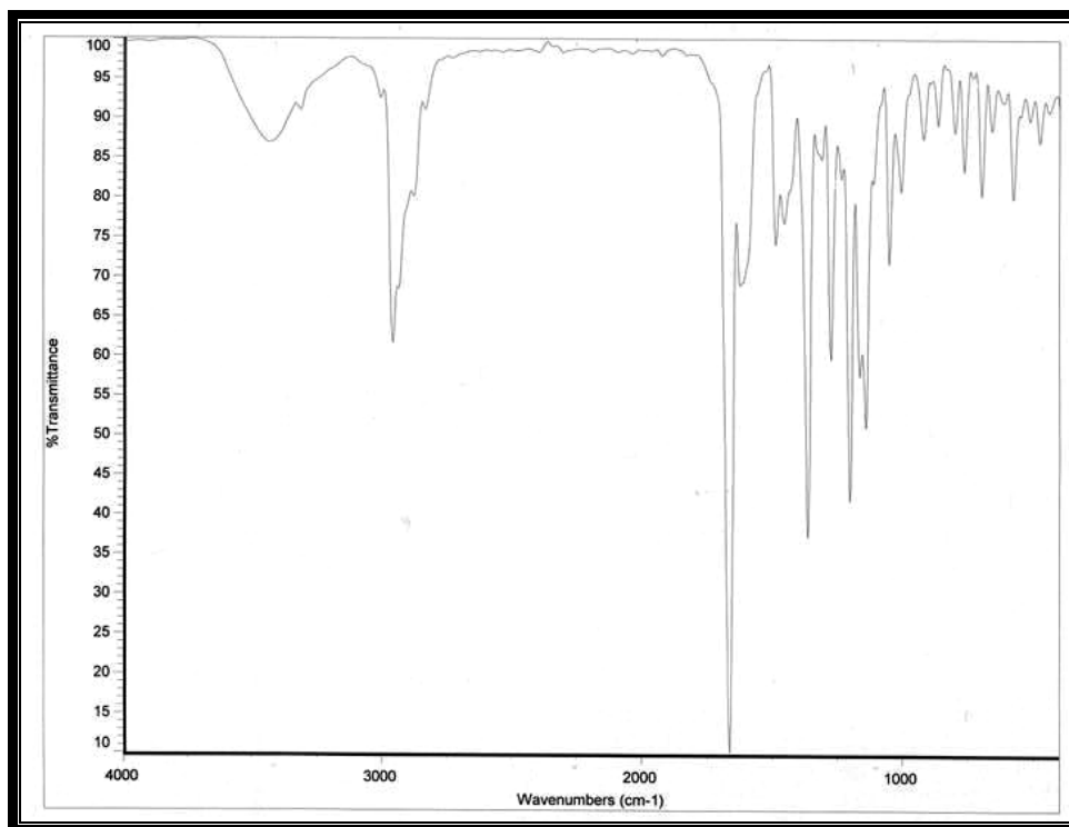
9-(4-Methoxy)-3,3,6,6-tetramethyl-1,2,3,4,5,6,7,8-octahydroanthene-1,8-dione:
