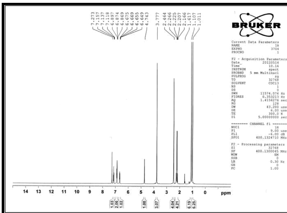
9-(3-Methoxy)-3,3,6,6-tetramethyl-1,2,3,4,5,6,7,8-octahydroanthene-1,8-dione:
