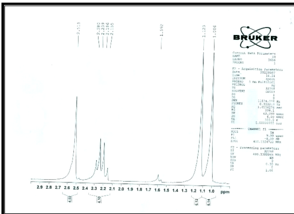
9-(3-Methoxy)-3,3,6,6-tetramethyl-1,2,3,4,5,6,7,8-octahydroanthene-1,8-dione:
