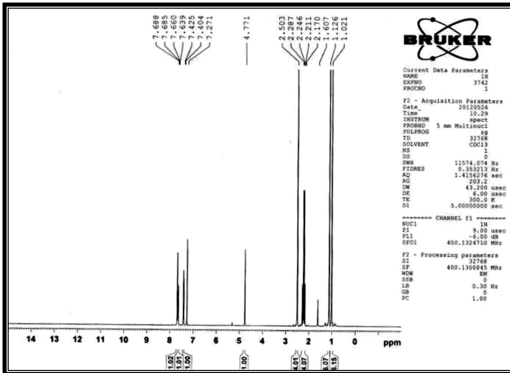
9-(4-Chloro-3-nitrophenyl)-3,3,6,6-tetramethyl-1,2,3,4,5,6,7,8-octahydroxanthene-1,8-dione:
