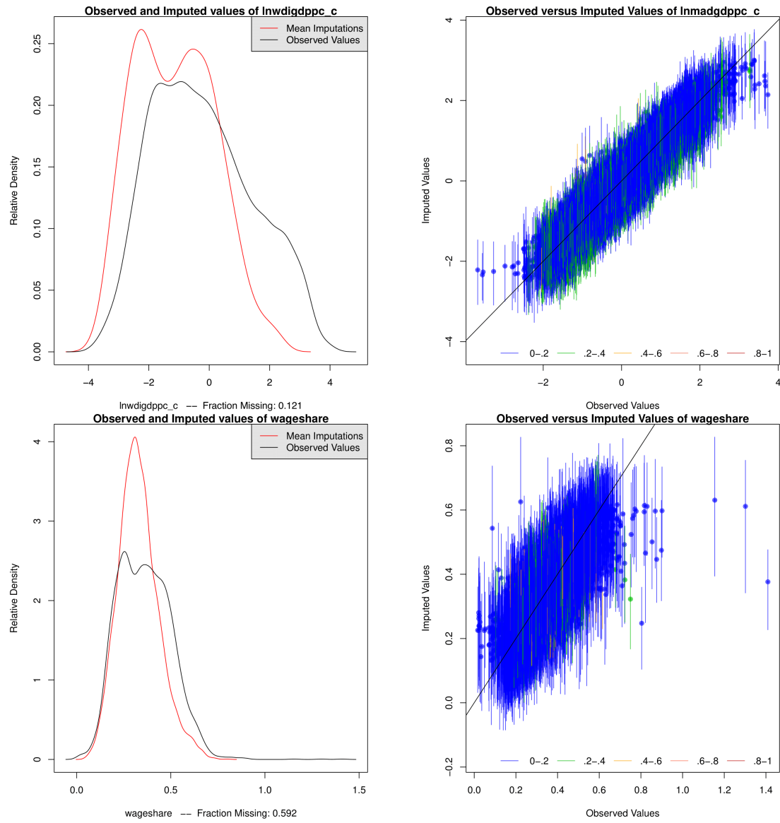
Figure 1: Density and overimputation plots for variables lnwdigdppc_c (top) and wageshare (bottom)
