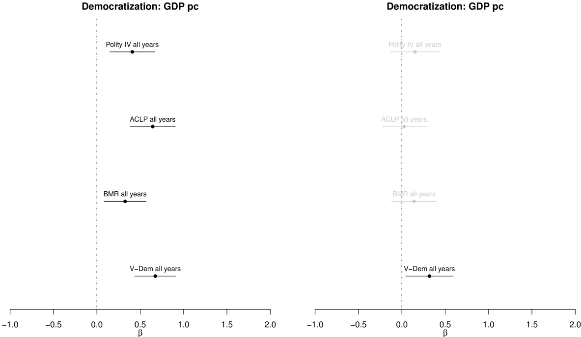
Figure 4: Within- (left) and between-country (right) coefficients for GDP pc and democratization controlling for natural resources. Black = significant at .05 level. Dark grey = significant at .10 level. Grey = insignificant.
