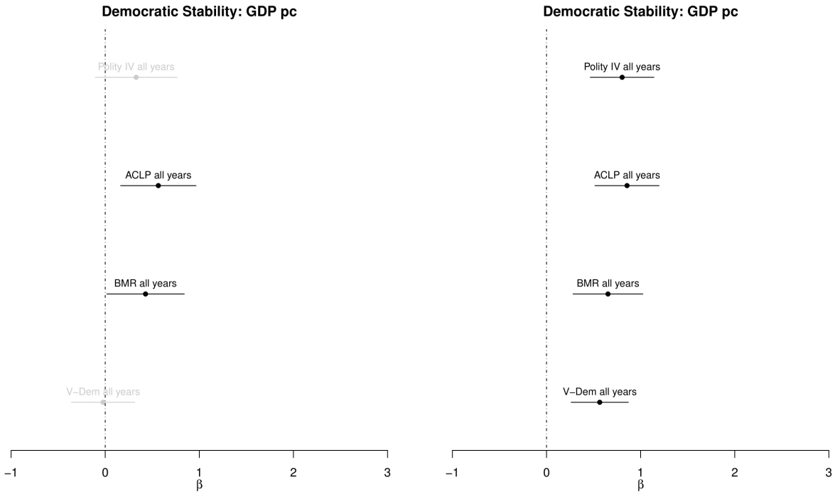
Figure 3: Within- (left) and between-country (right) coefficients for GDP pc and democratic stability, all specifications. Black = significant at .05 level. Dark grey = significant at .10 level. Grey = insignificant.
