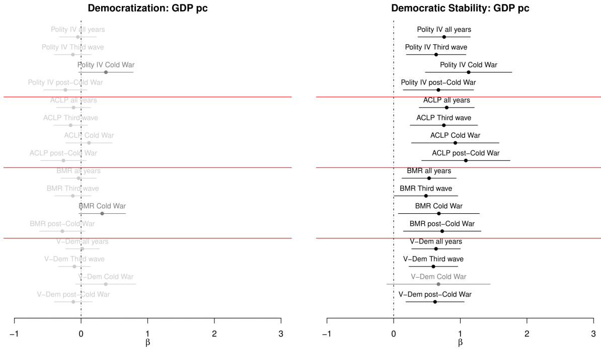
Figure 5: Coefficient plots of \bar{\beta} with 95% C.I. across all specifications for GDP pc (Bolt et al. 2018) and democratization (left) and GDP pc on democratic stability (right). Black = significant at .05 level. Dark grey = significant at .10 level. Grey = insignificant.
