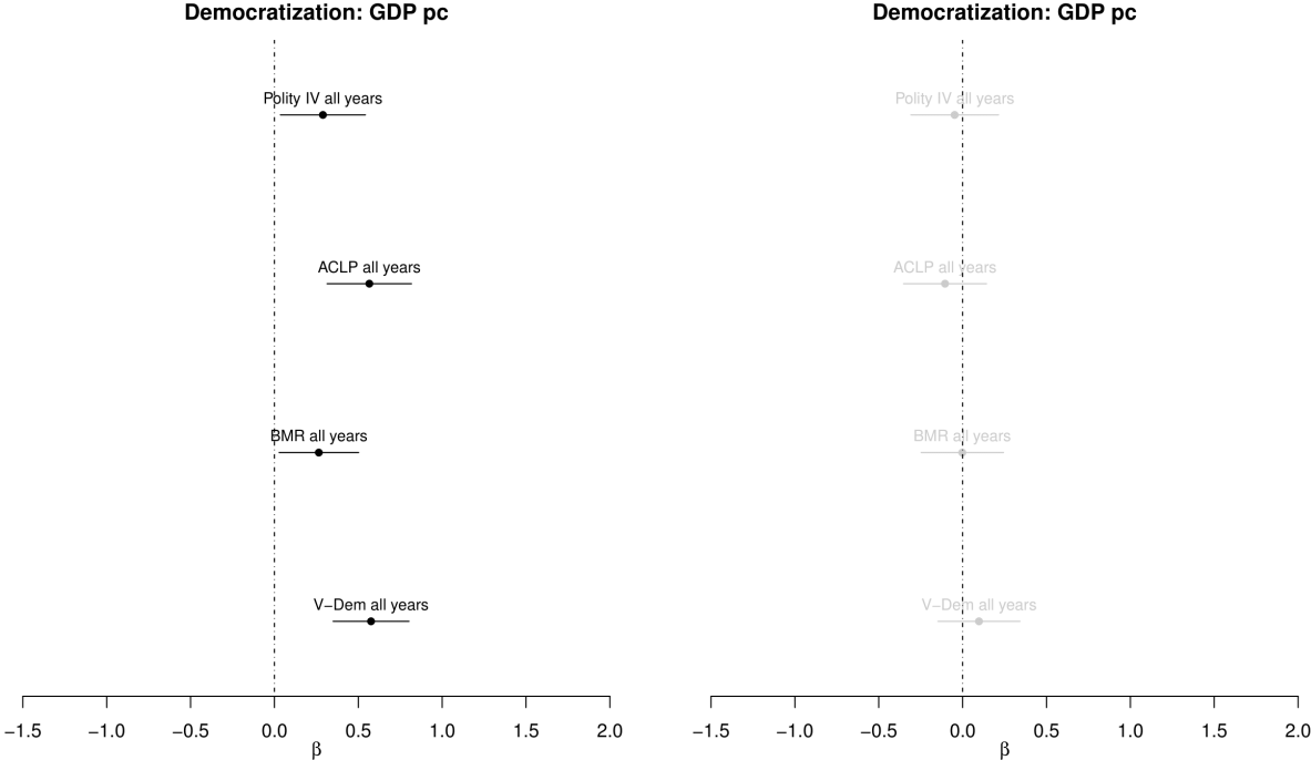
Figure 2: Within- (left) and between-country (right) coefficients for GDP pc and democratization, all specifications. Black = significant at .05 level. Dark grey = significant at .10 level. Grey = insignificant.
