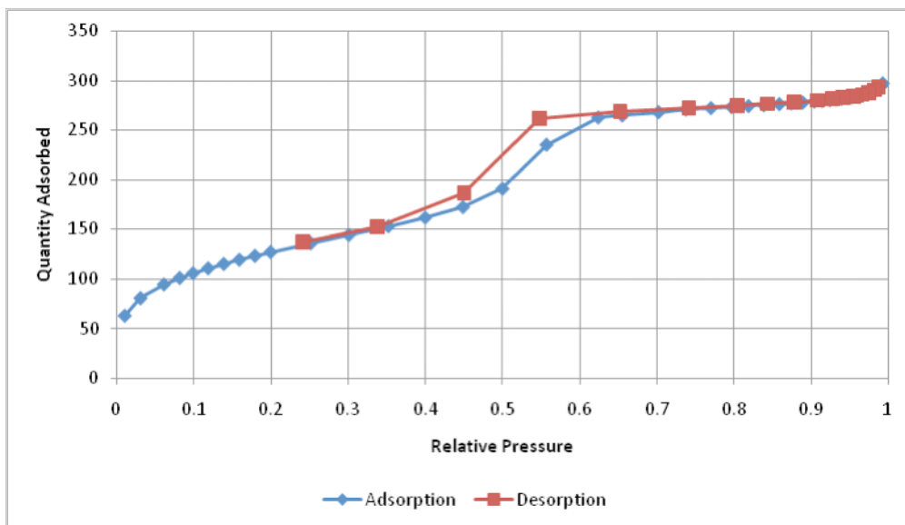
Figure S2. N 2 Adsorption/Desorption Isotherms for Tp-SBA-15
