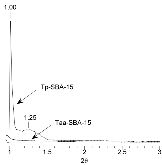
Figure S1. Low angle XRD of Tp-SBA-15 and Taa-SBA-15
