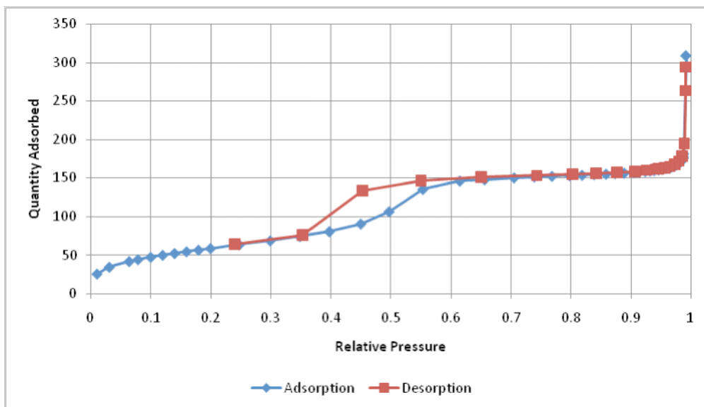
Figure S3. N 2 Adsorption/Desorption Isotherms for Taa-SBA-15
