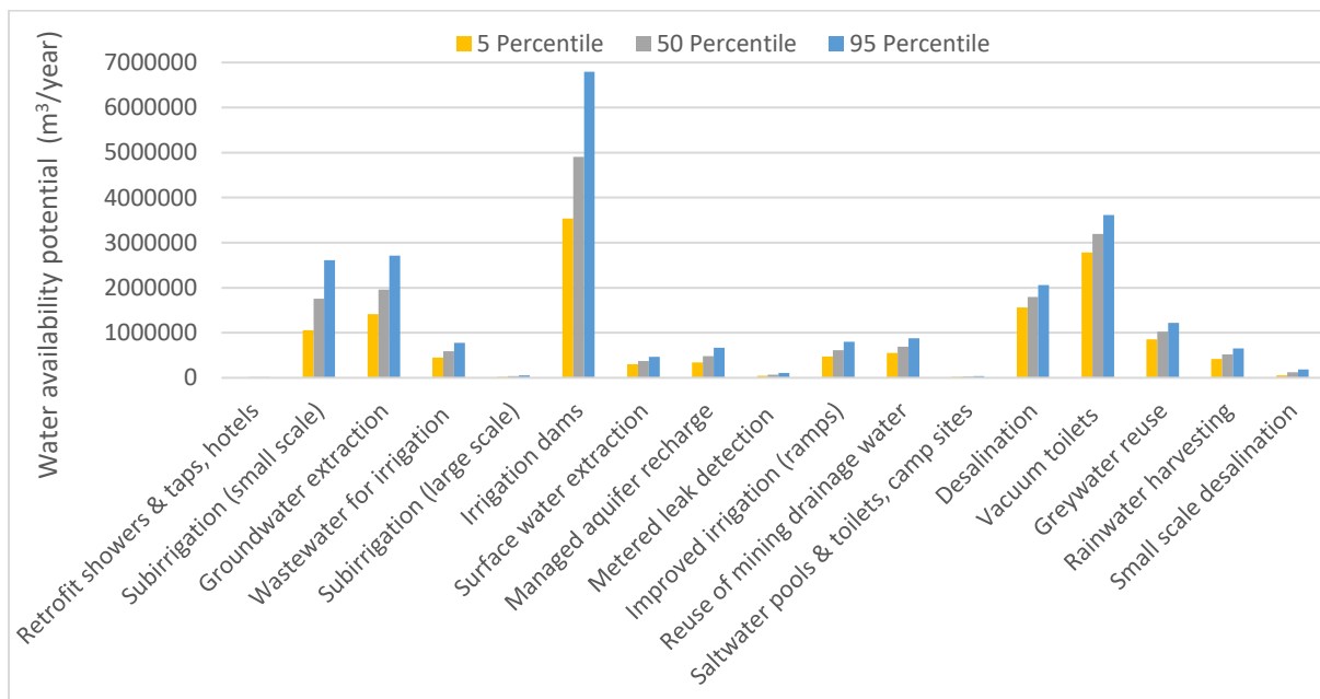
Fig 1 Water availability potential for all analyzed measures, percentiles P05, P50 and P95
