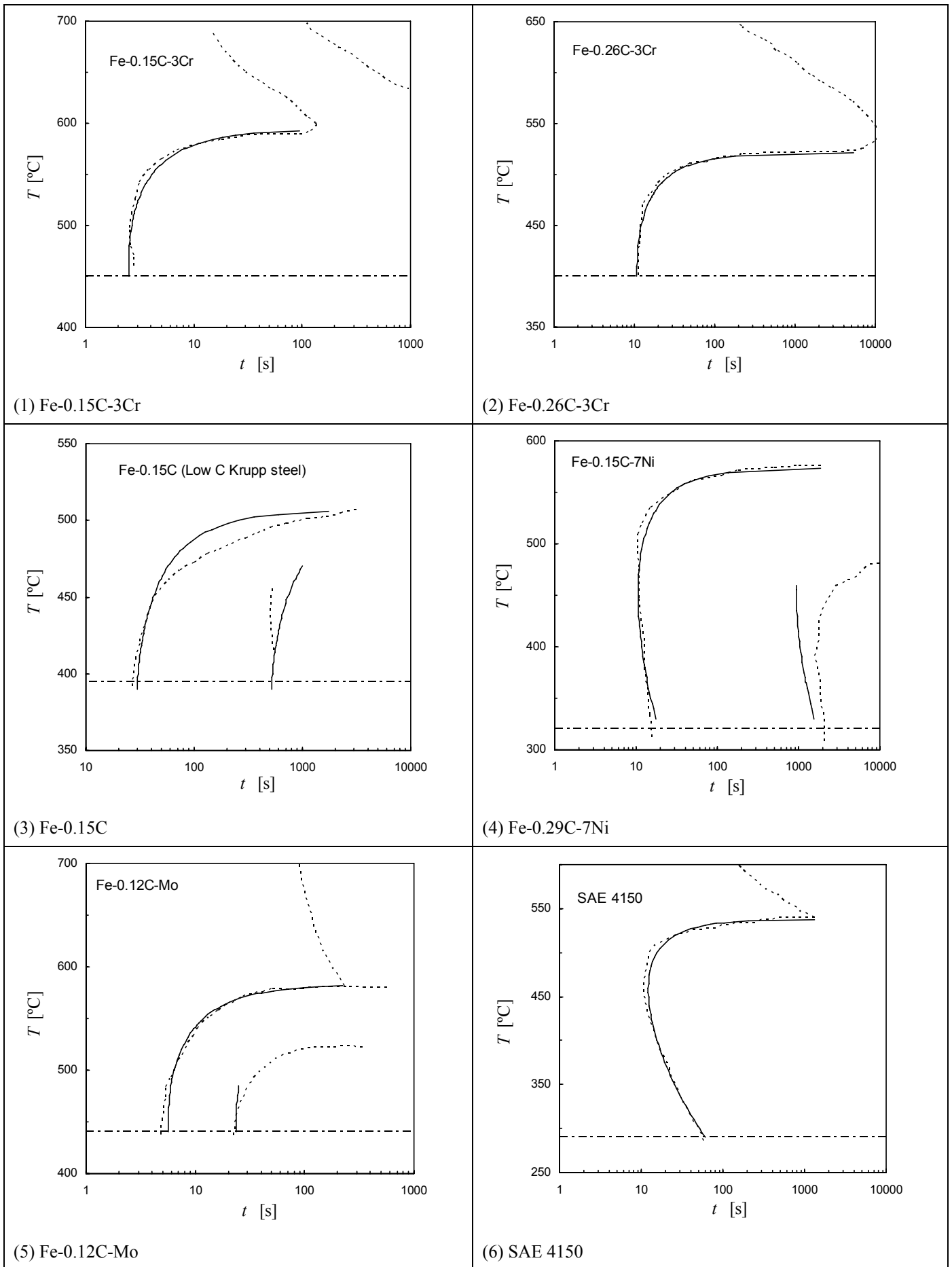
Figure 1. Alloys 1 - 6: experimental (dotted line) and calculated (solid line) start-curves.
