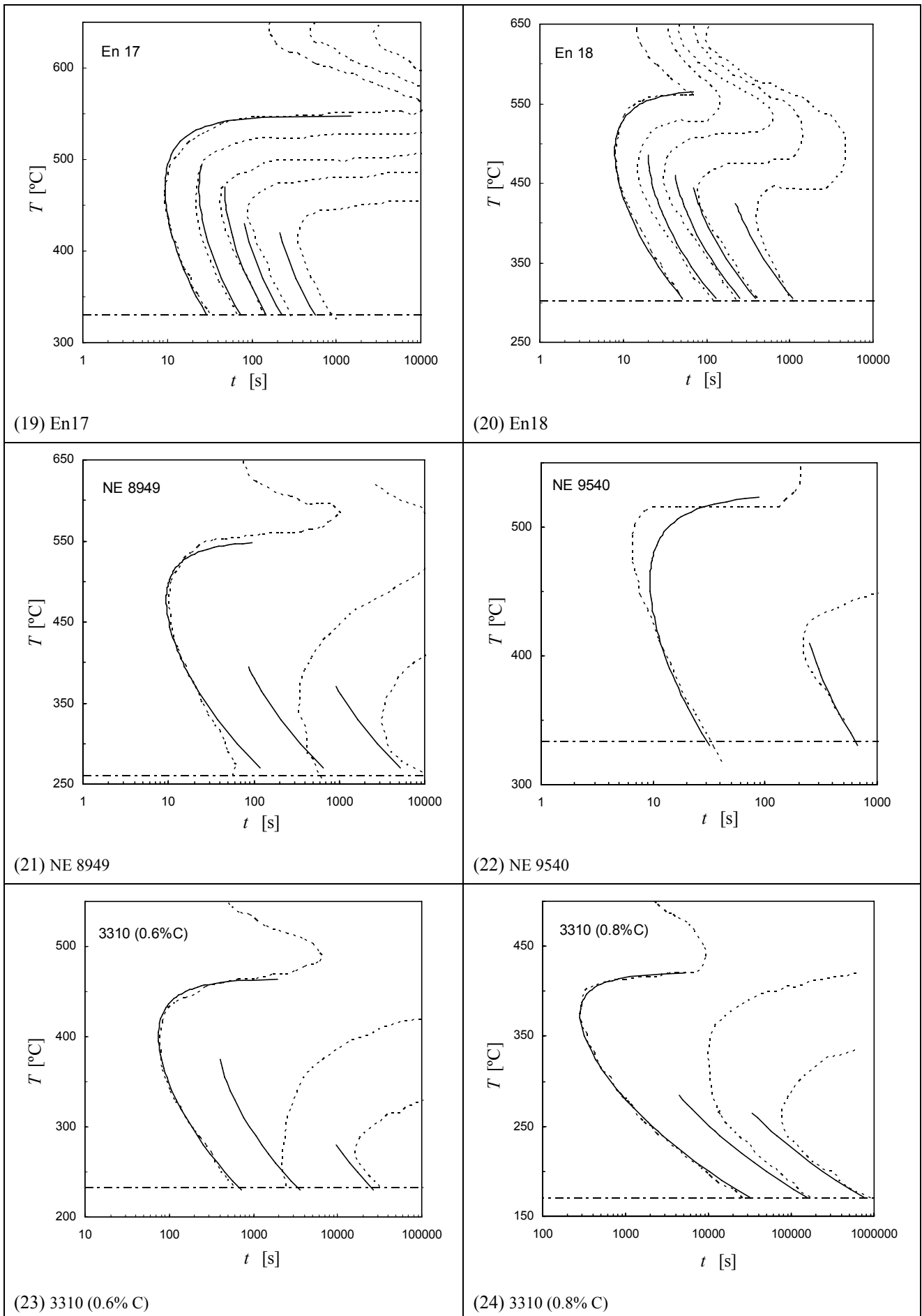
Figure 4. Alloys 19 - 24: experimental (dotted line) and calculated (solid line) start-curves.
