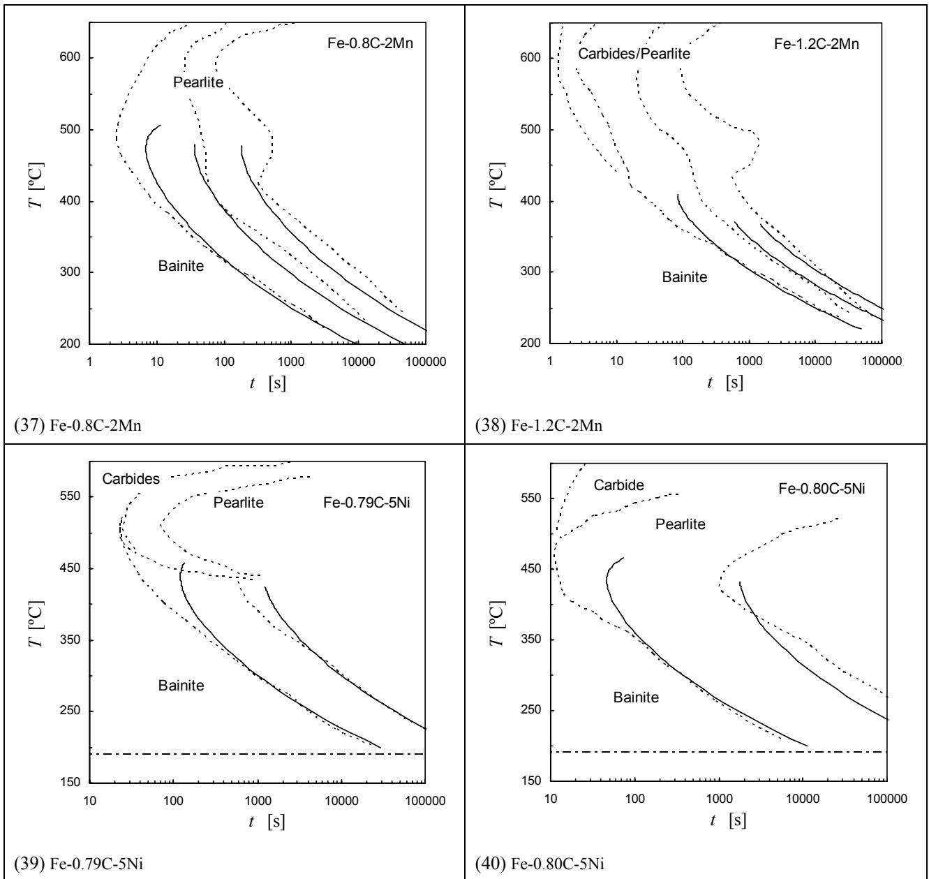
Figure 7. Alloys 37 - 40: experimental (dotted line) and calculated (solid line) start-curves.
