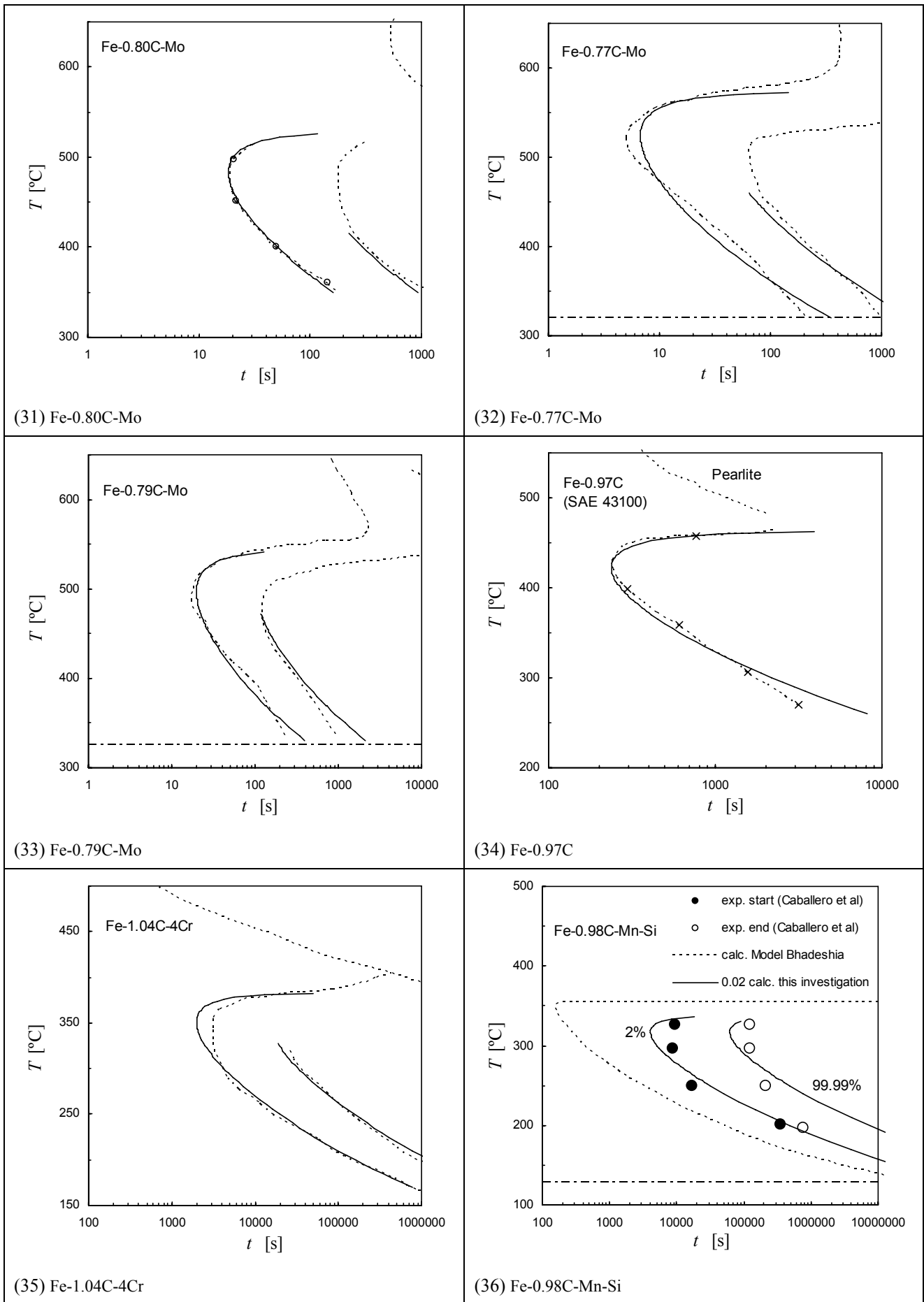
Figure 6. Alloys 31 - 36: experimental (dotted line) and calculated (solid line) start-curves.
