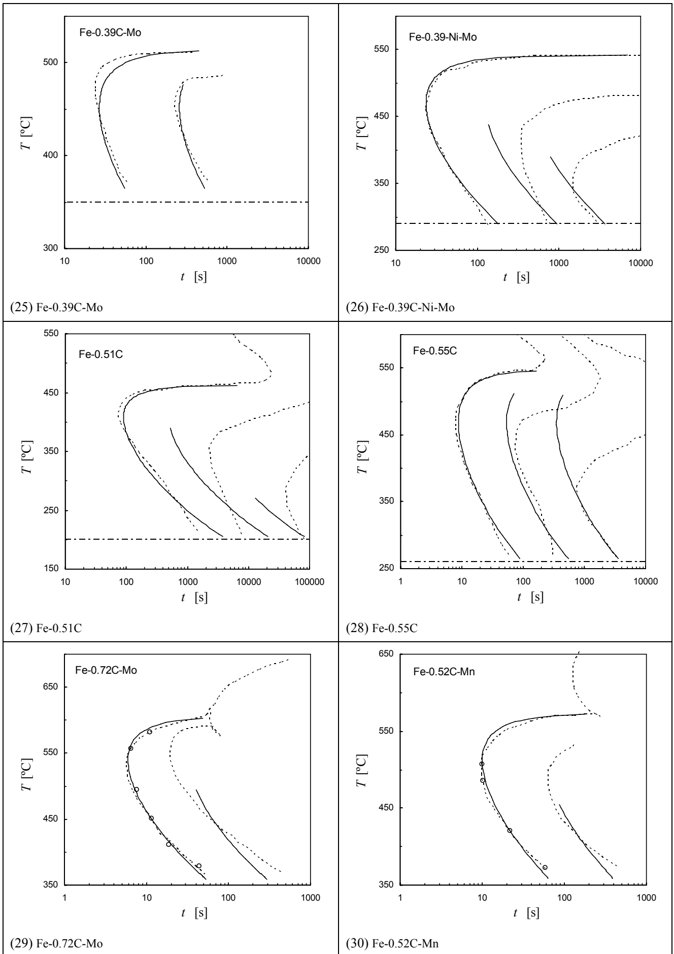
Figure 5. Alloys 25 - 30: experimental (dotted line) and calculated (solid line) start-curves.
