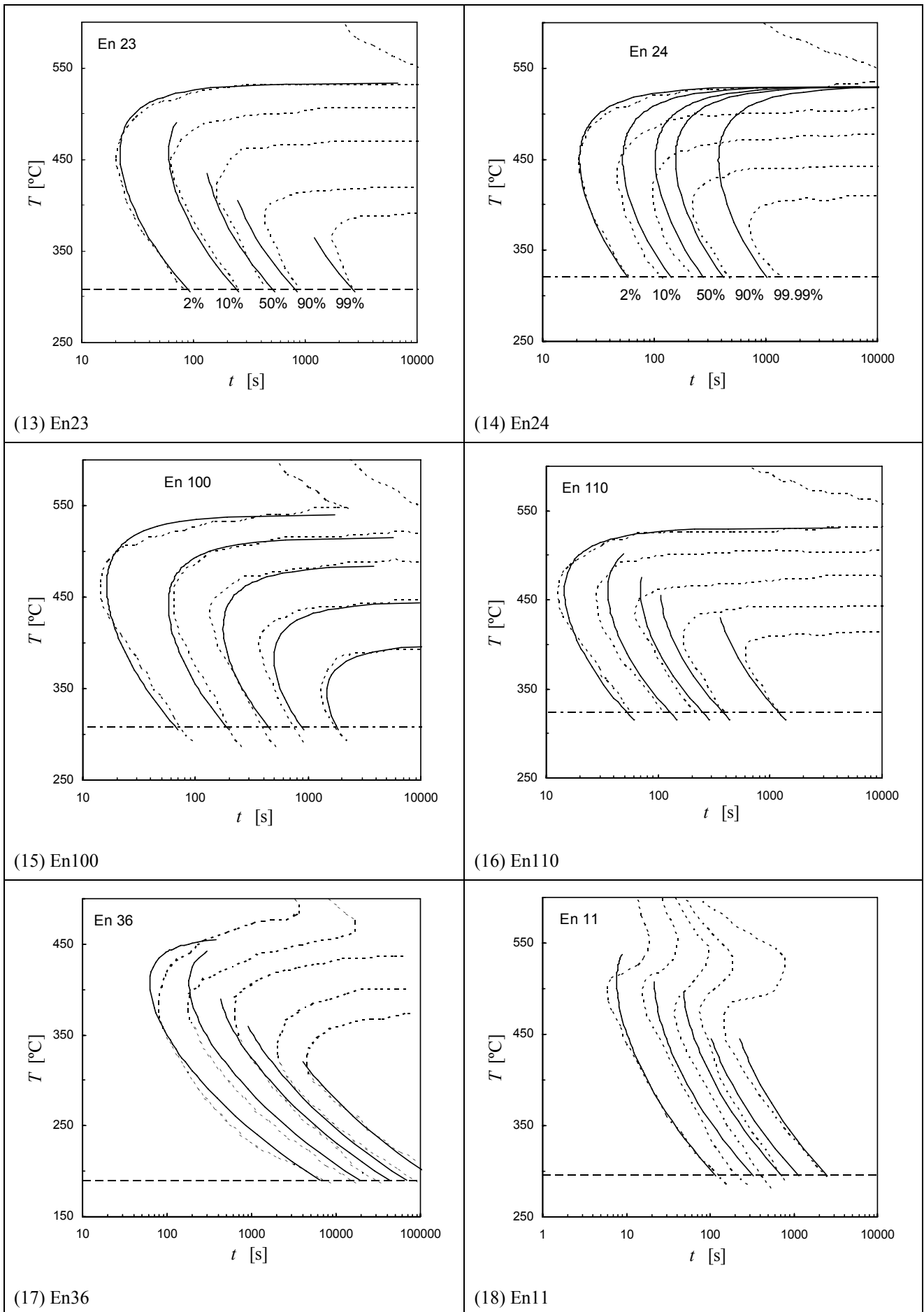
Figure 3. Alloys 13 - 18: experimental (dotted line) and calculated (solid line) start-curves.
