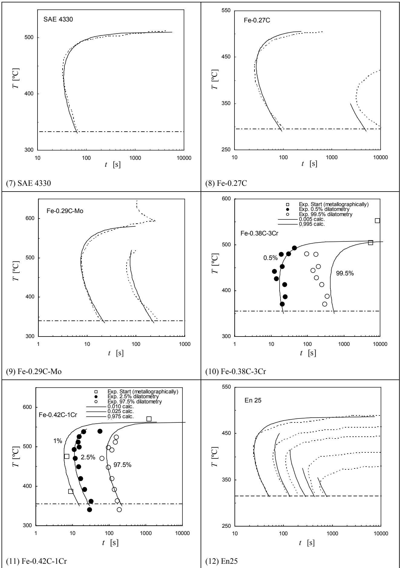
Figure 2. Alloys 7 - 12: experimental (dotted line) and calculated (solid line) start-curves.
