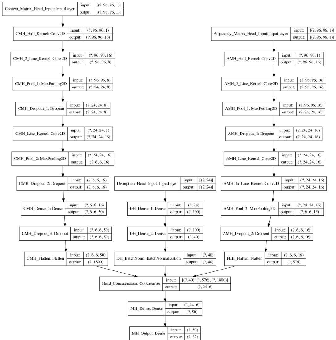
Figure 6: Visualization of the three-headed NN structure for disruption type classification. ? refers to the TensorFlow representation for the chosen batch-size of 32.
