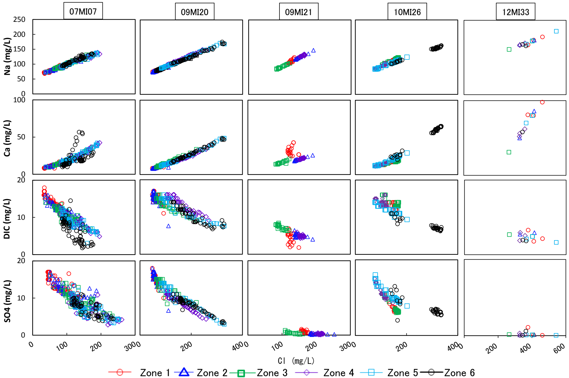
Fig. Relationship of chloride and other chemical components concentrations in the galleries.
