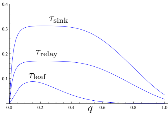
(a) Configuration A: 7 leaves at each of the 2 relays ( N_1 = 7, N_2 = 2 ).
