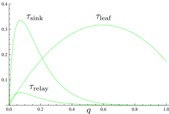
(c) Configuration C: 1 leaf at each of the 8 relays ( N_1 = 1, N_2 = 8 ).
