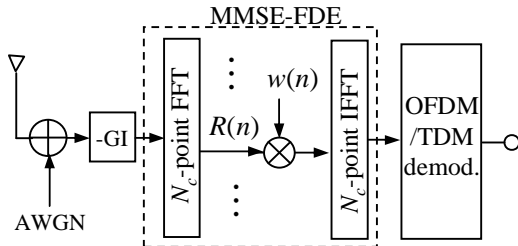
(b) Receiver
