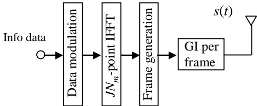
(a) Transmitter
