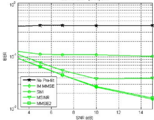
BER for SIR = (-5 dB) 3TX
