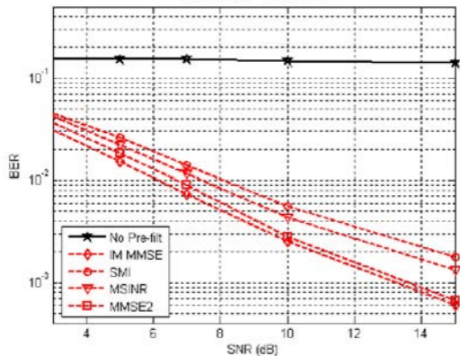
BER for SIR = (-5 dB) 2TX
