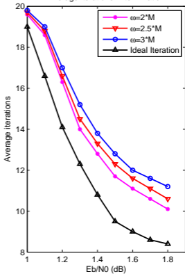
Average iterations in termination
