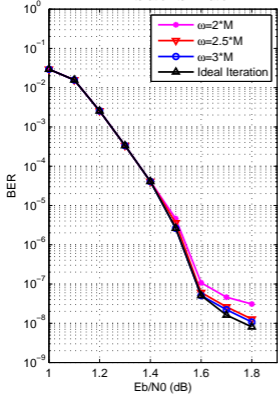
BER in iteration termination
