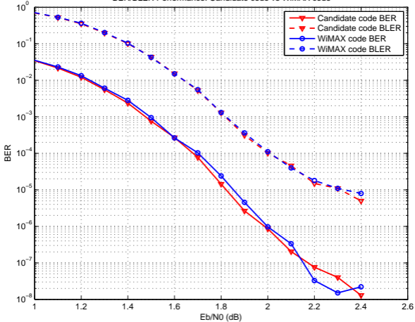
BER/BLER Performance: Candidate code vs WiMAX code
