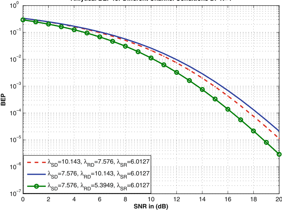
Analytical BEP for Different Channel Conditions DF N=4
