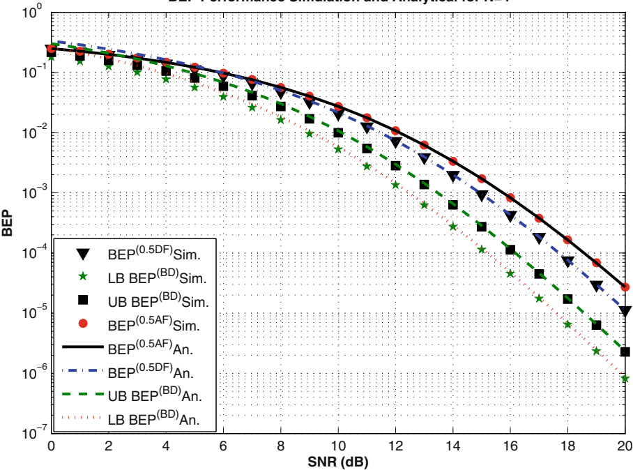
BEP Performance Simulation and Analytical for N=4
