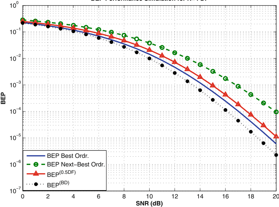
BEP Performance Simulation for N=4 DF
