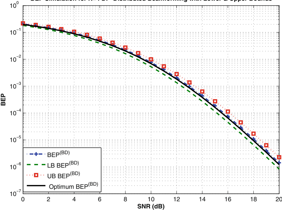
BEP Simulation for N=4 DF Distributed Beamforming with Lower & Upper Bounds
