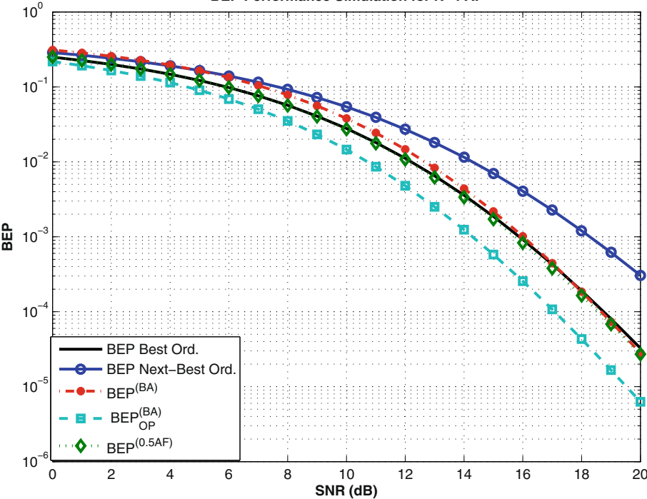
BEP Performance Simulation for N=4 AF
