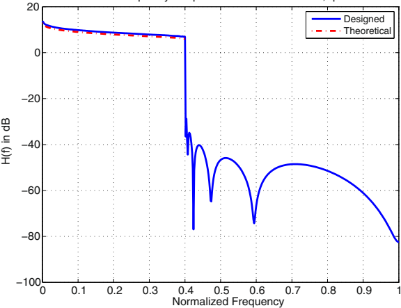
Frequency Response of IIR Filter For a=1 , q=0.5
