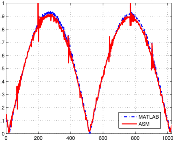
Normalized Absolute values MATLAB and Fixed Point Output
