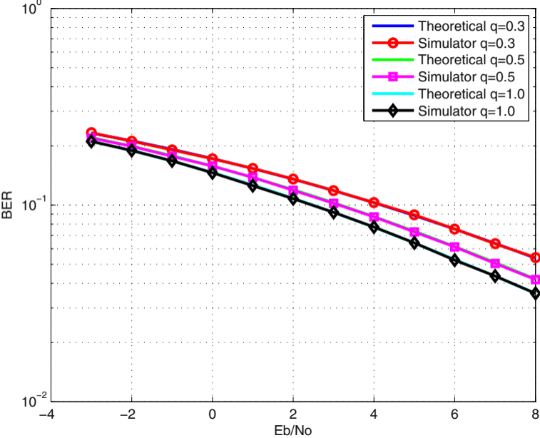
BPSK BER F_s=2e6 F_b=200e3
