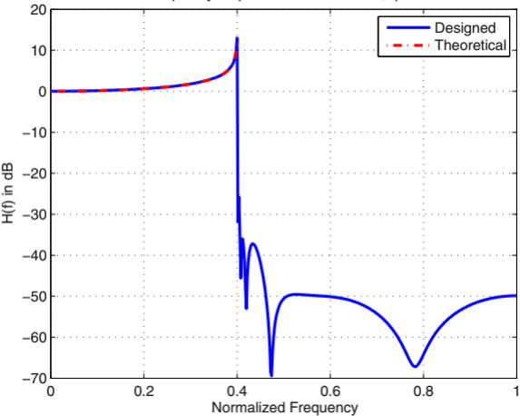
Frequency response of IIR Filter a=0 , q=0.5
