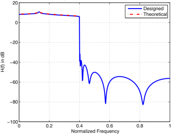
Frequency Response of IIR Filter For q=0.5 a=0.5
