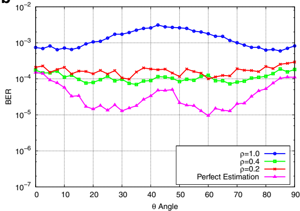
Phase Estimation Error (PLL algorithm used).
