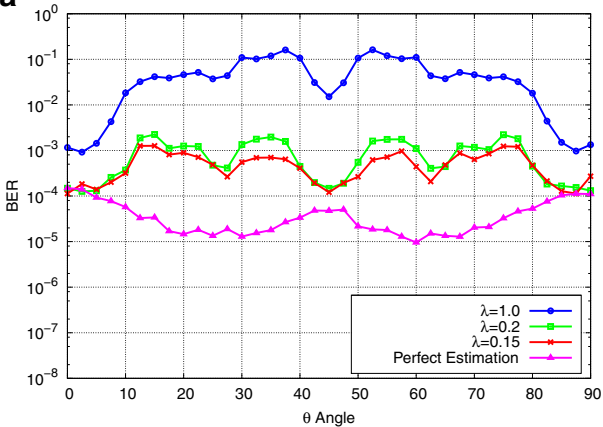
Amplitude Estimation Error (LMS algorithm used).
