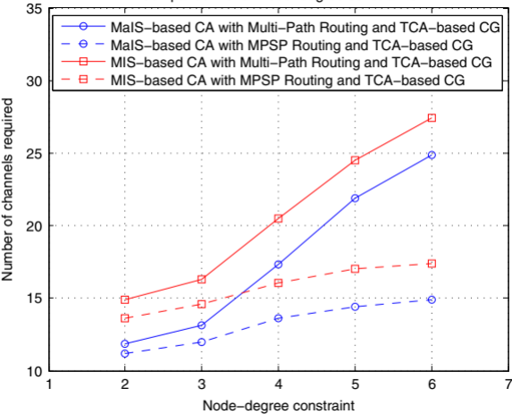
Comparison for all node-degree constraints
