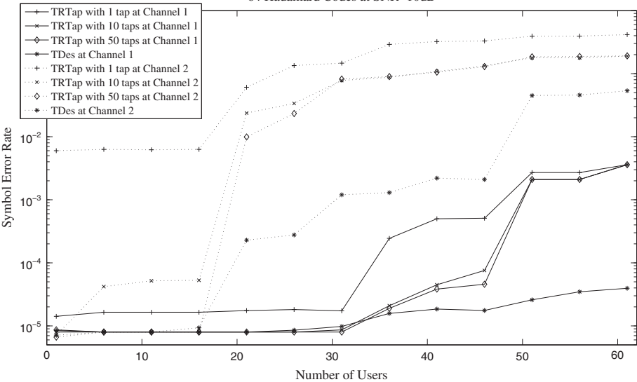
64 Hadamard Codes at SNR=10dB
