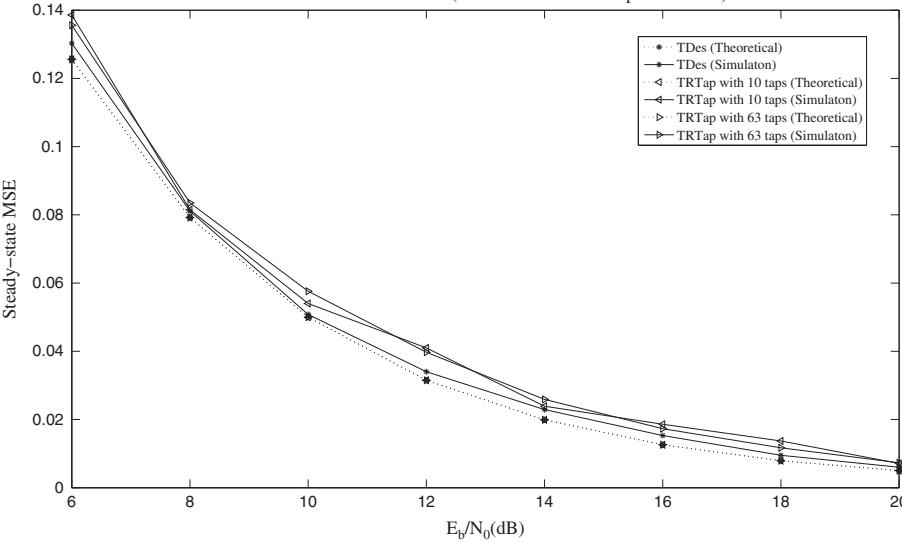
Simulation v.s. Theoretical (30 users without multipath channel)
