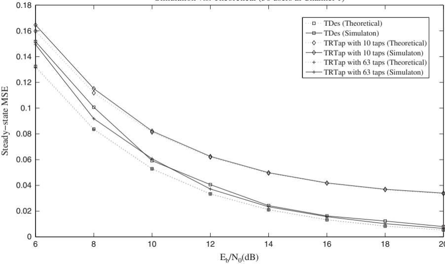
Simulation v.s. Theoretical (30 users at Channel 1)
