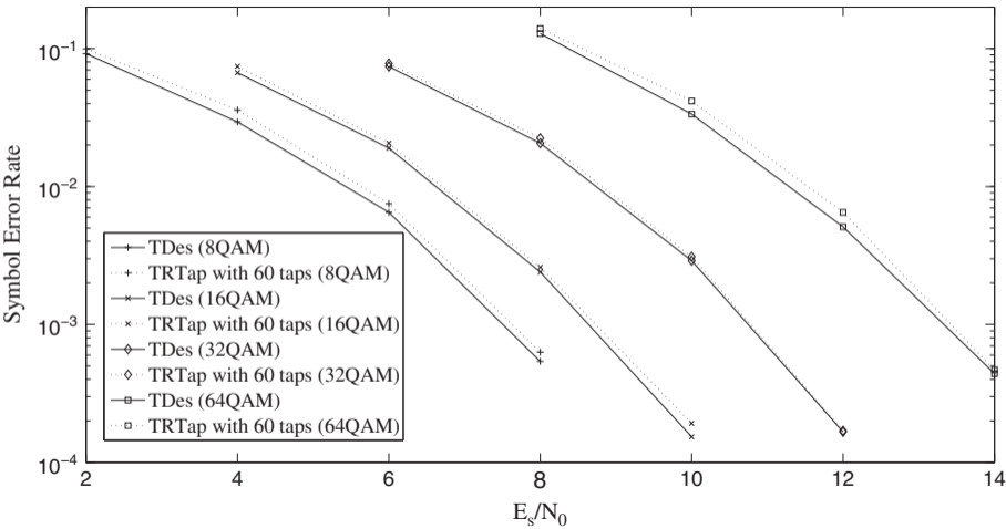
64 Hadamard Codes with 10 users at Channel 1
