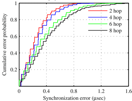
Multi-hop synchronization error of R-RS
