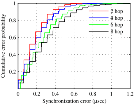
Multi-hop synchronization error of TTS
