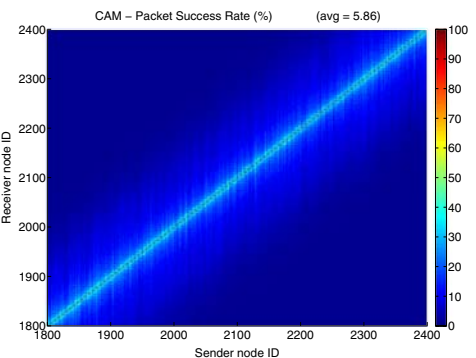
(a) CAM PSR characteristics
