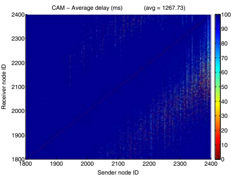
(b) CAM delay characteristics
