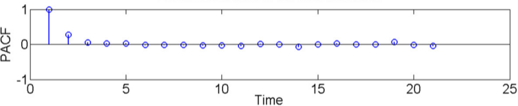
Partial correlation of the second difference
