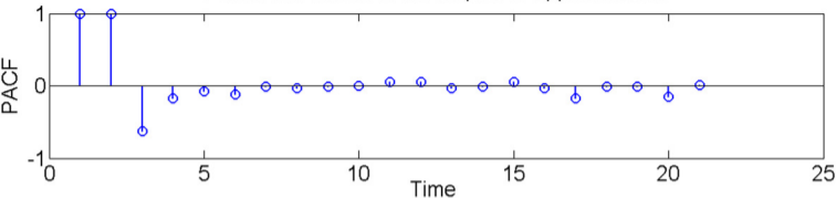
Partial correlation of the first difference
