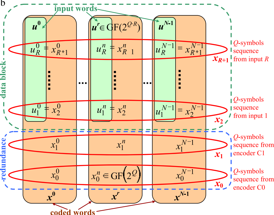
Q -symbol-level structure of MNB turbo coded block;
