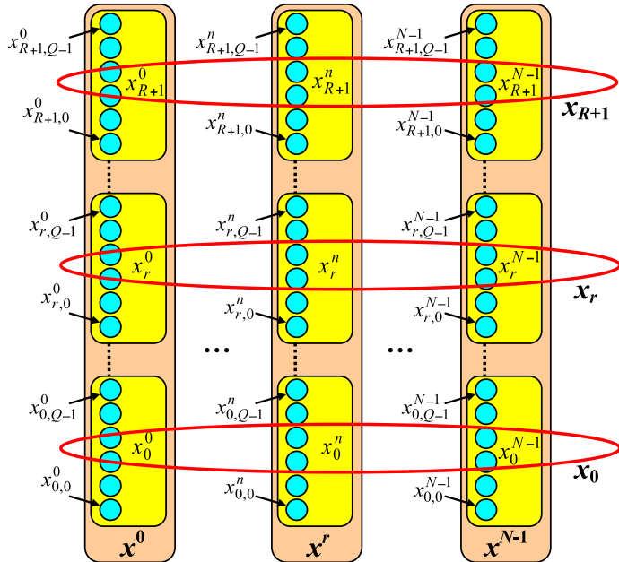
bit-level structure of MNB turbo coded block;
