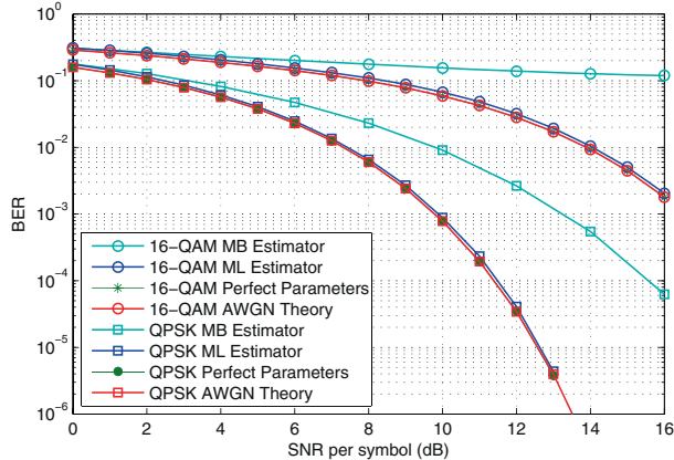
(b) M-QAM
