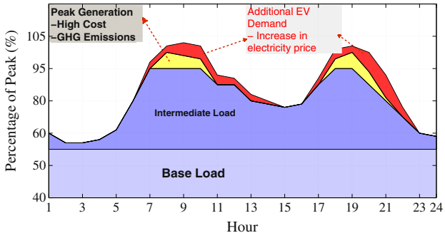
Typical Utility Daily Curve
