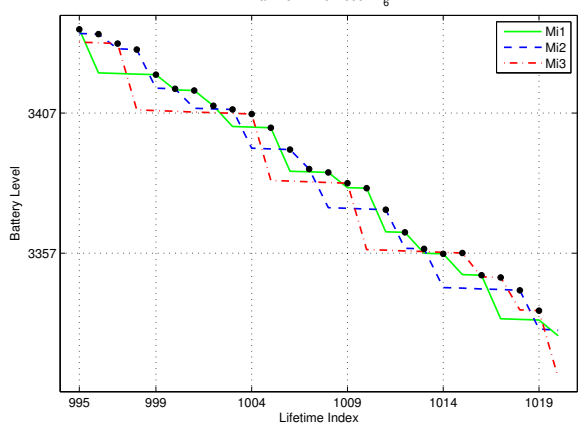
Maximum Likelihood : H_6
