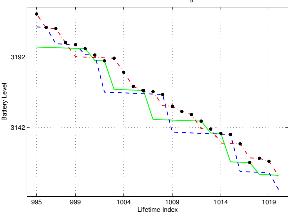
Maximum Likelihood : H_5
