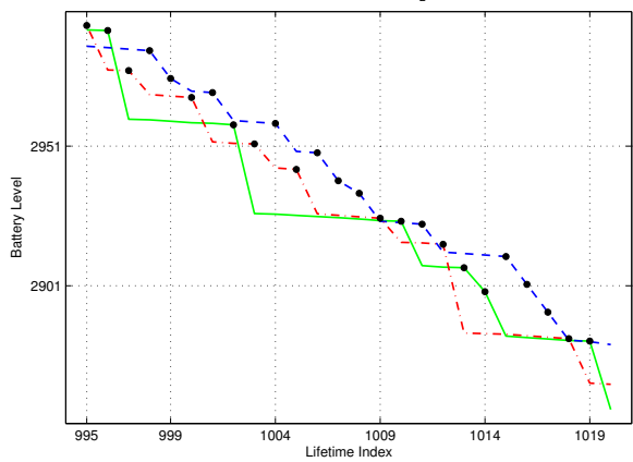
Maximum Likelihood : H_4
