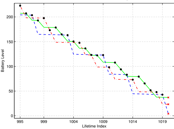
Maximum Likelihood : H_3
