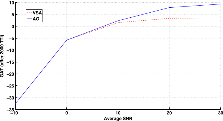
Performance Comparison of Centralized and Distributed Solution at Various SNR Regimes
