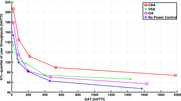
Average Cell-Edge User Throughput VS. Geometric Mean, Fast-Fading
