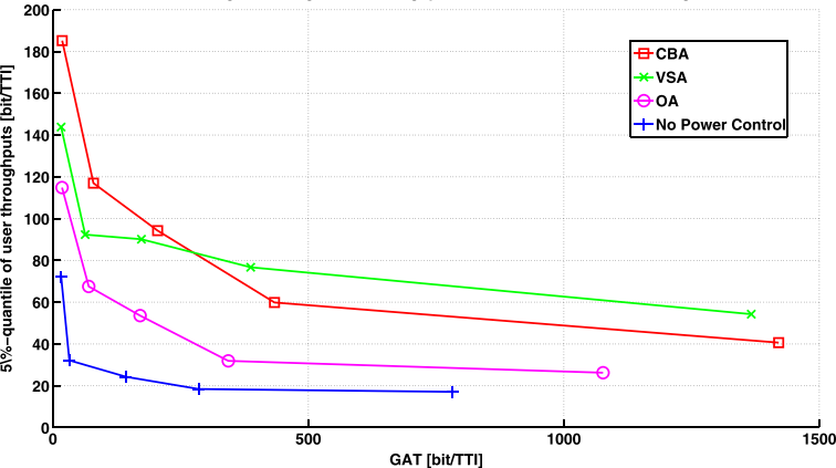
Average Cell-Edge User Throughput VS. Geometric Mean, No Fading
