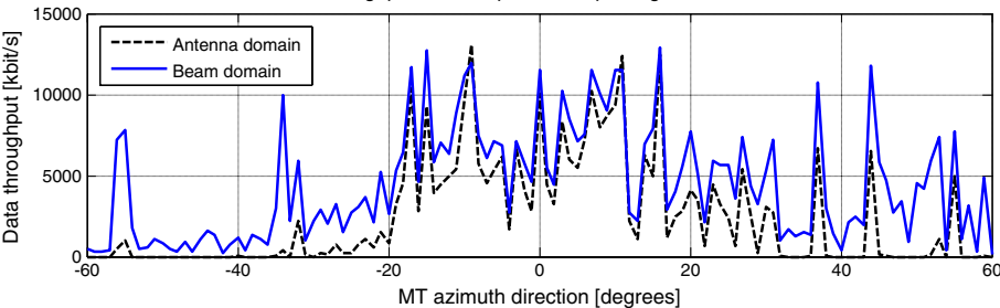
Total throughput of 2x2 Spatial Multiplexing with 64QAM-1/2
