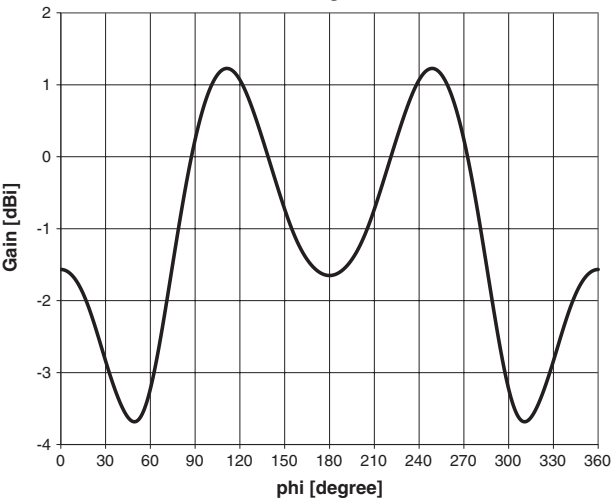
Beam pattern 1
