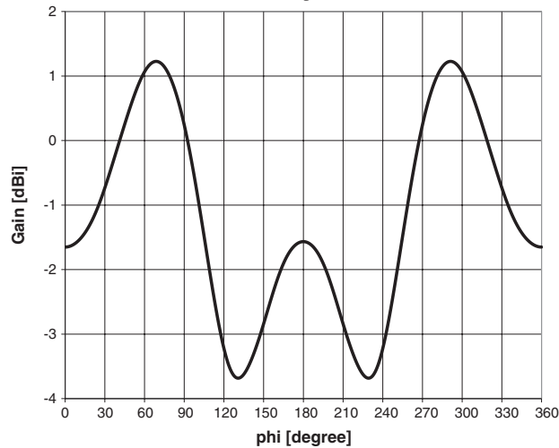
Beam pattern 2
