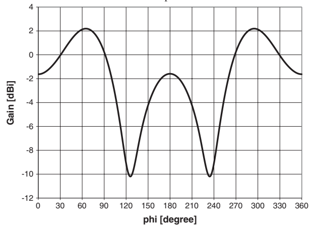
Beam pattern 2
