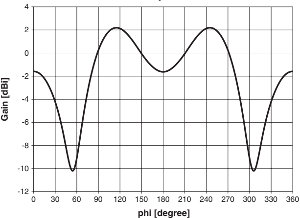
Beam pattern 1
