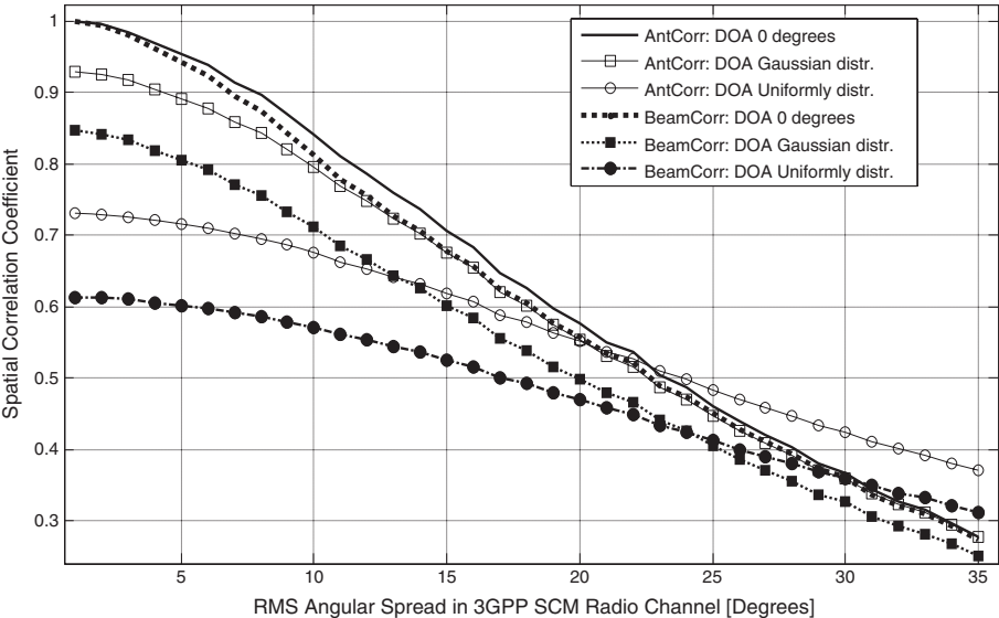
Spatial Correlation in Antenna and beam Domains
