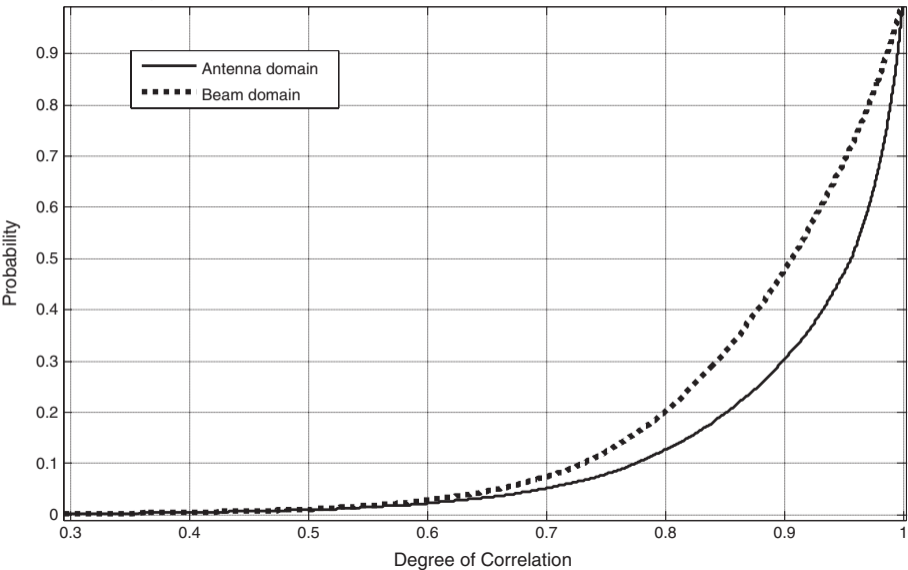
Empirical CDF of MIMO channel correlation in Simulated ITU Pedestrian B Radio Channel
