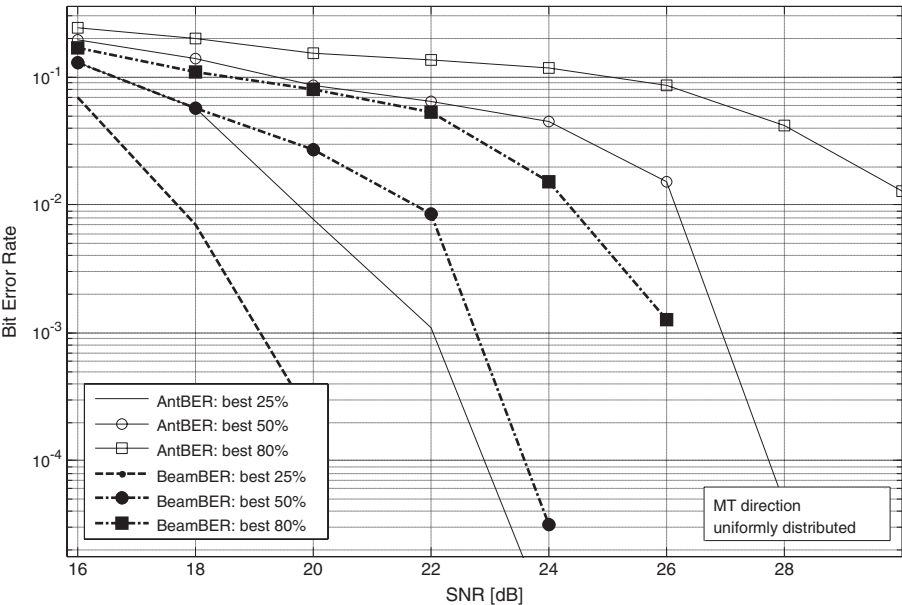
BER Performance of 2x2 Spatial Multiplexing with Turbocoded 64QAM-1/2
