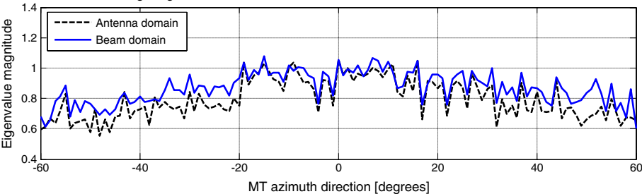
Average Eigenvalues of 2x2 MIMO channel matrices for 10 best resource blocks
