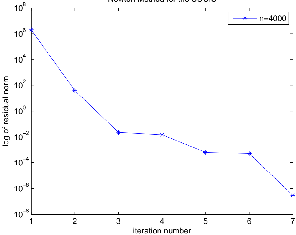
Newton Method for the SOCIS
