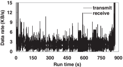
Master node
