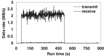
Reduce node
