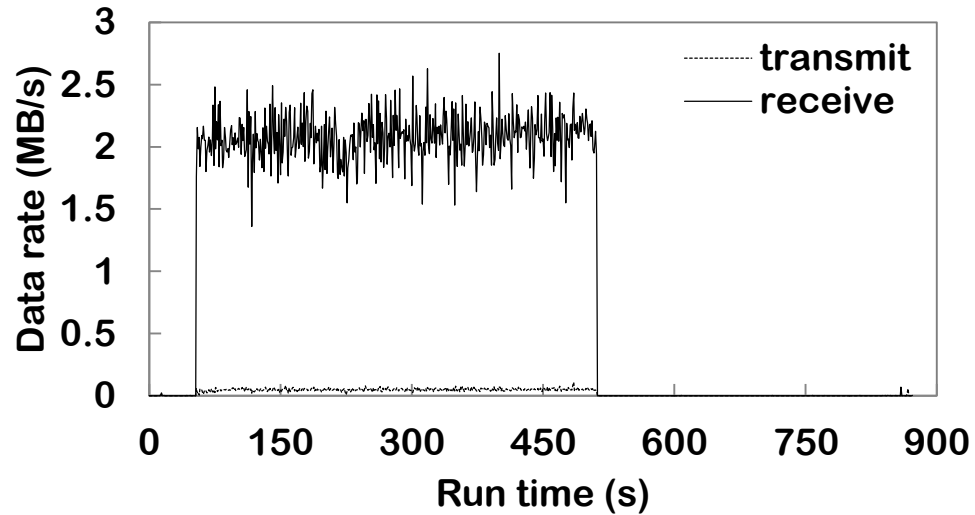
Reduce node
