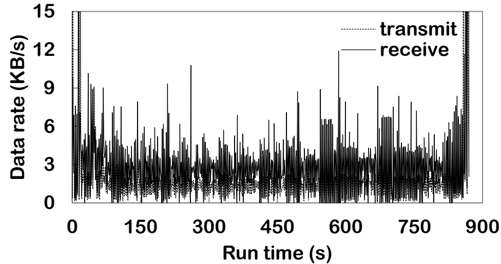
Master node
