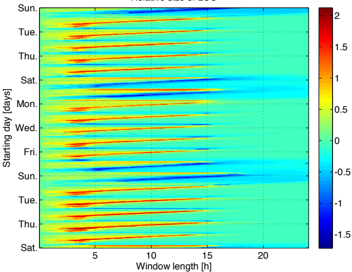
Relative size of LCC
