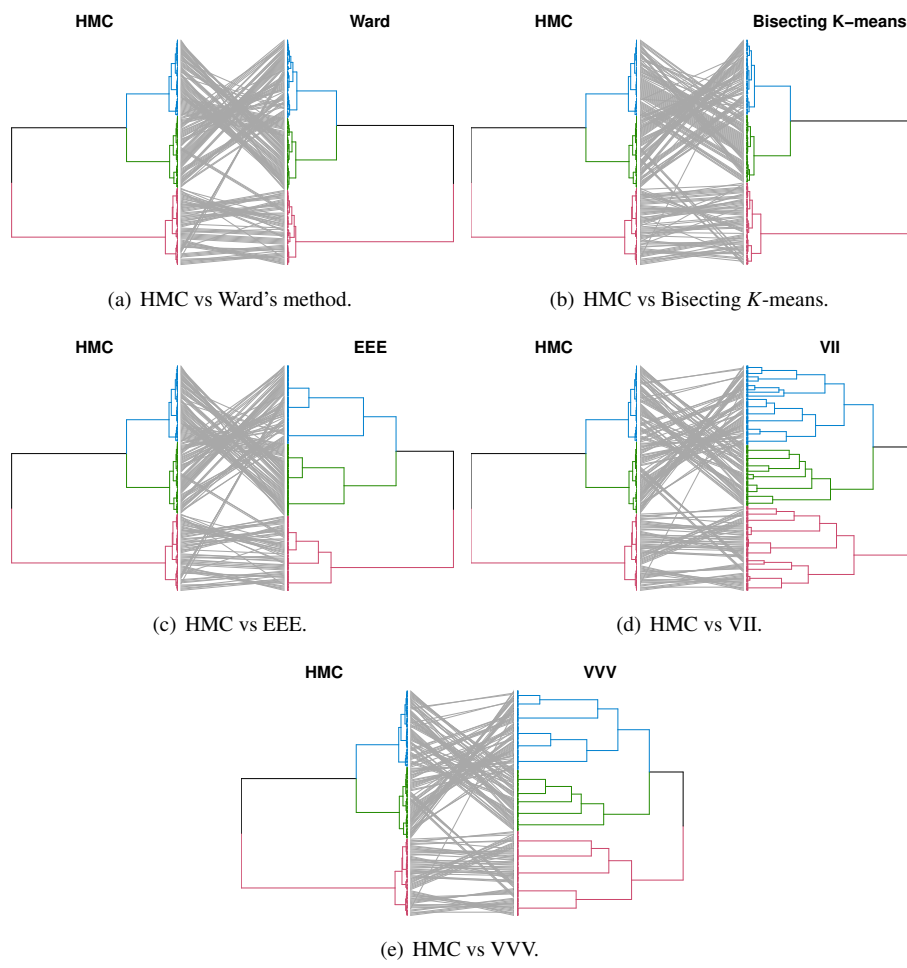
Fig. A.5: Seeds data: comparison between dendrograms.
