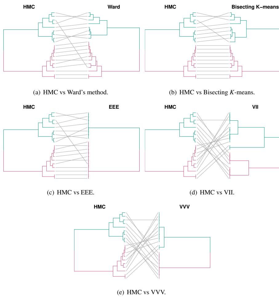
Fig. A.1: Archaeology data: comparison between dendrograms.
