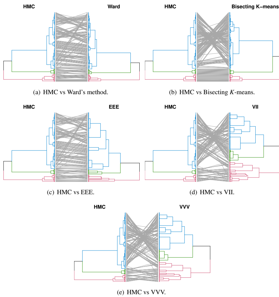
Fig. A.4: Thyroid data: comparison between dendrograms.
