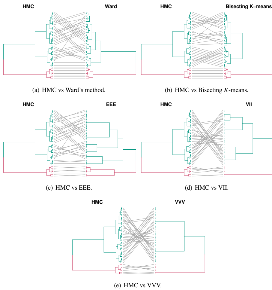
Fig. A.2: Coffee data: comparison between dendrograms.
