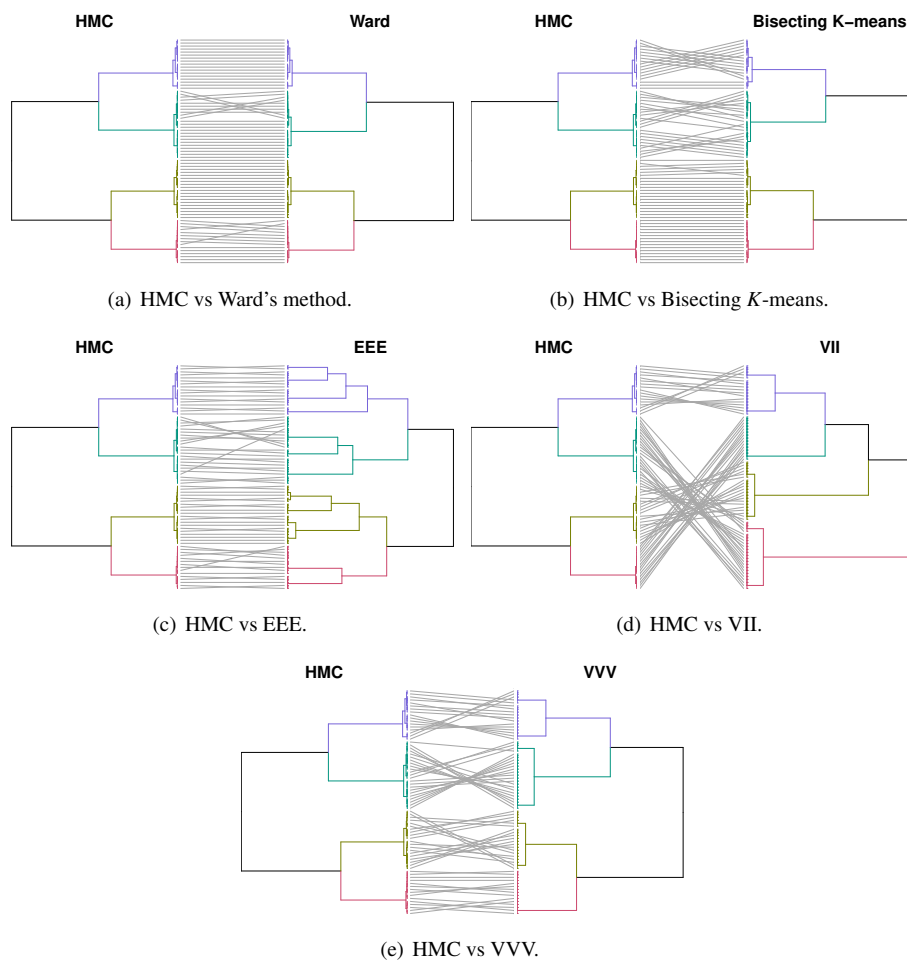
Fig. A.3: Ruspini data: comparison between dendrograms.
